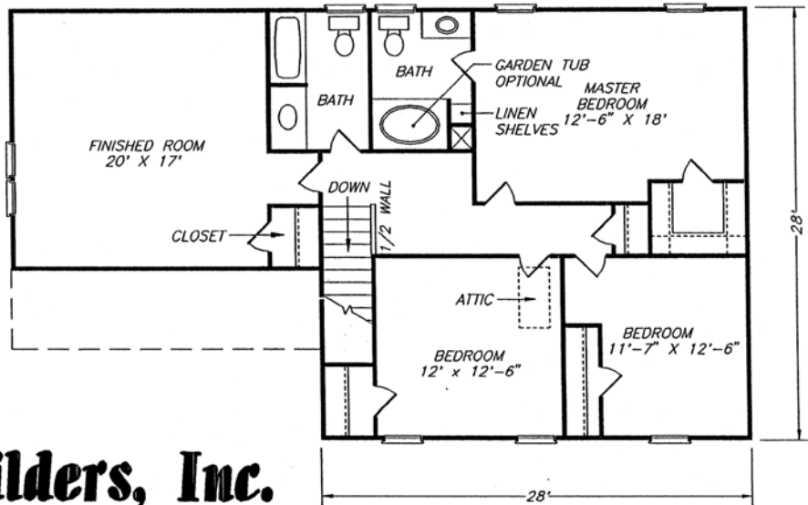
SECOND FLOOR
