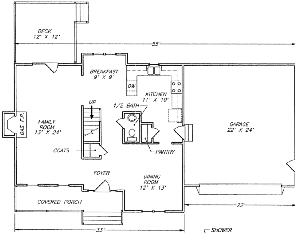
FIRST FLOOR
